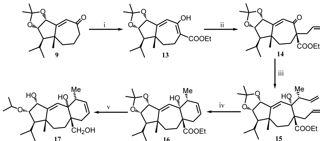
Scheme 2. Reagents and conditions: (i) LDA, THF-HMPA, CNCOOEt, -78°C, 75%; (ii) NaH, THF, allyl bromide, rt, 95%; (iii) Mg, 3-chloro-1-butene, CeCl 3 , THF, 60%; (iv) Grubbs' catalyst (10 mol%), benzene, Δ, 96%; (v) DIBAL-H, DCM, 65%.
